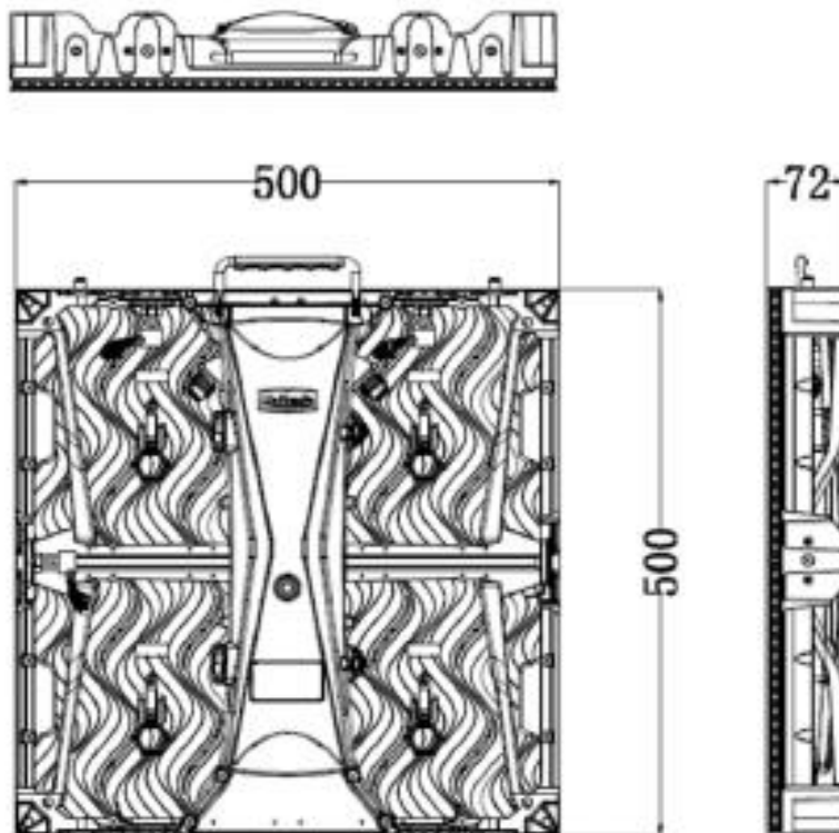
Figure1 Cabinet Drawing
