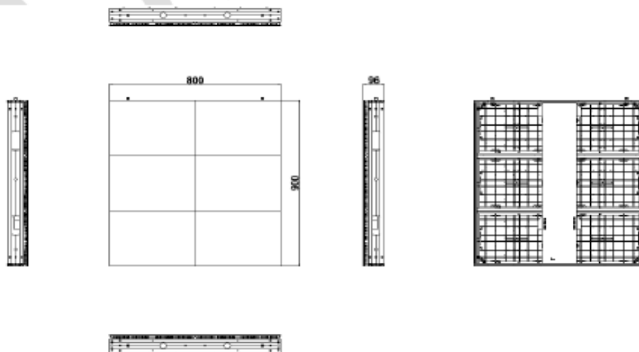
Figure 2 Drawing of Rear Maintenance Cabinet
