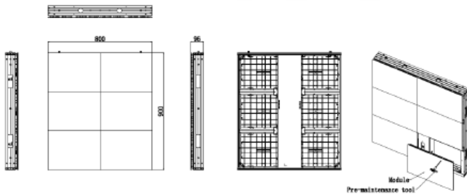
Figure 1 Drawing of Front Maintenance Cabinet
